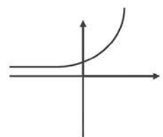
Exponential Graph Of form y = a^x
